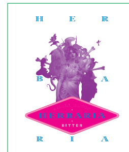
EMBOSS
